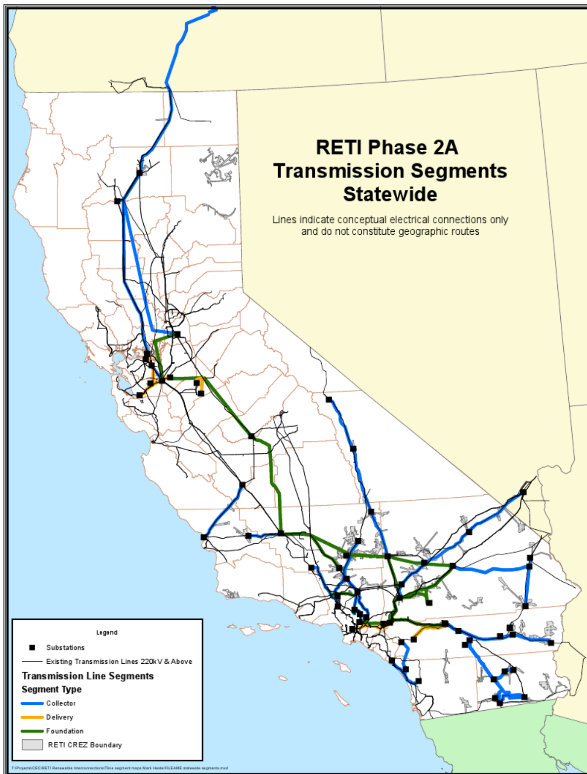
Figure 1-2. Foundation Lines, Delivery Lines and Renewable Collector Lines.
