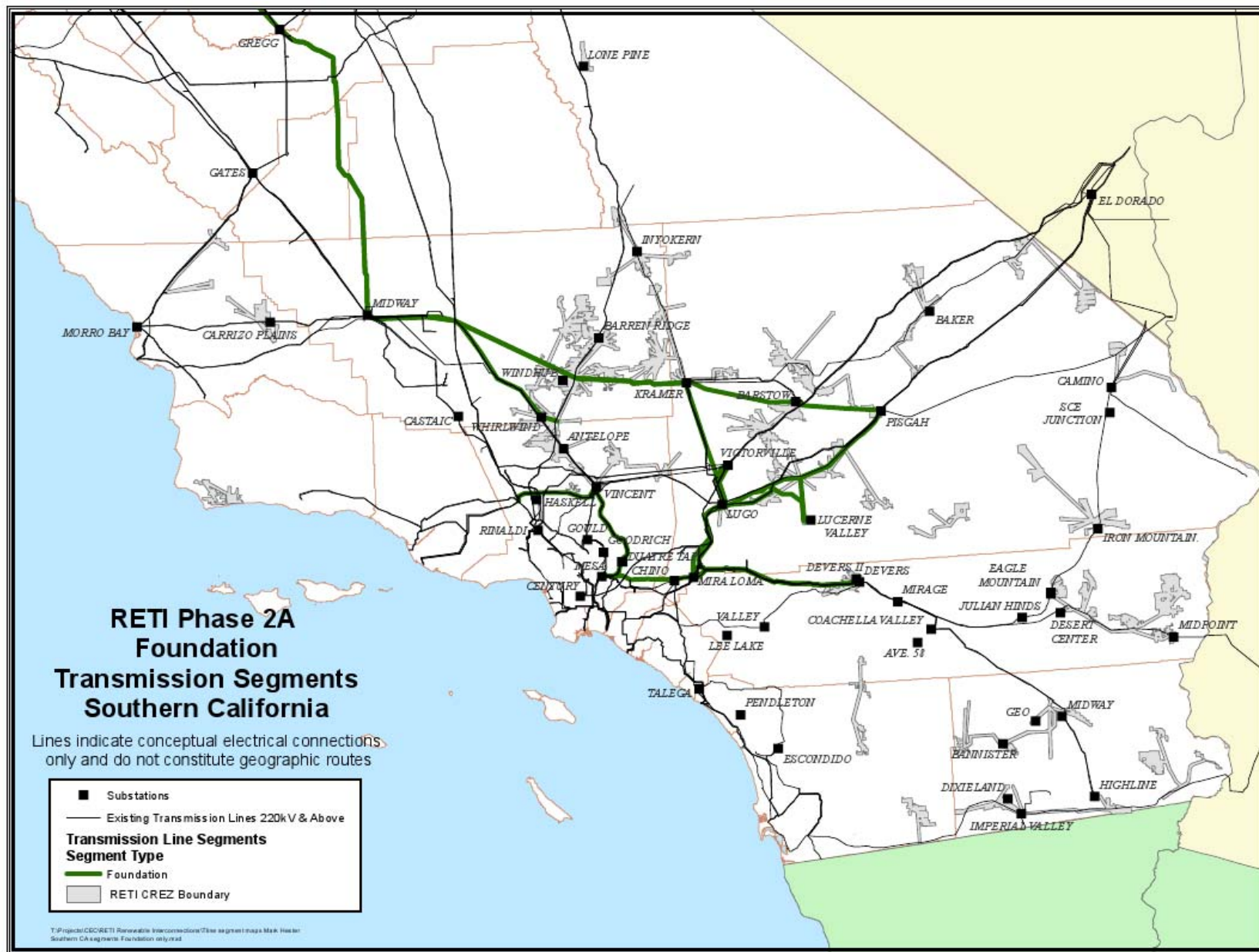
Figure 3-4. Map of Southern California Foundation Group Segments.
